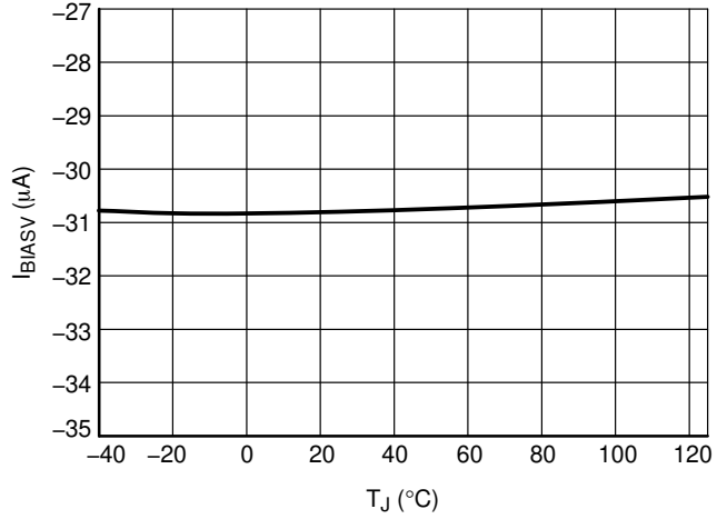
Figure 9. I BIASV at V CC = 15 V, V SNS > V SNSBIASV , V EC0DET < 10% V CC
