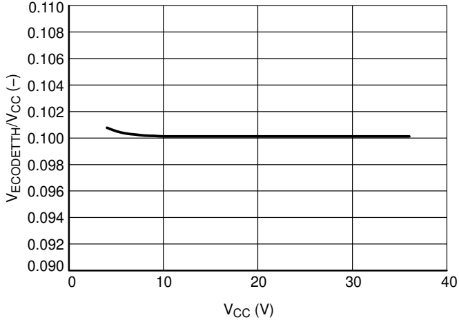
Figure 8. V EC0DETH /V CC Ratio at T J = 25°C
