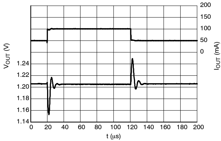
Figure 29. Load Transients, 1.2 V Version, I OUT = 50 – 100 mA, t R = t F = 0.5 μs, V IN = 2.6 V
