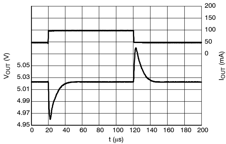
Figure 31. Load Transients, 5.0 V Version, I OUT = 50 – 100 mA, t R = t F = 0.5 μs, V IN = 6.0 V
