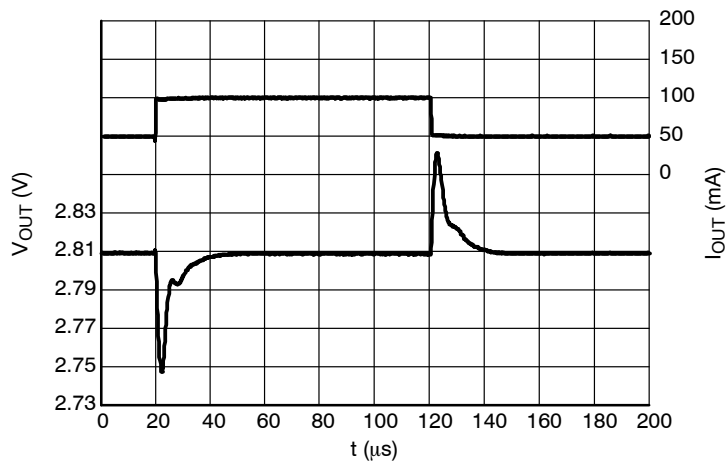
Figure 30. Load Transients, 2.8 V Version, I OUT = 50 – 100 mA, t R = t F = 0.5 μs, V IN = 3.8 V
