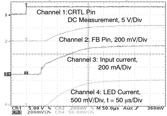
Figure 13. Startup for 3 LEDs Operating, I LEDs : 100 mA, R sense = 2.5 Ω
