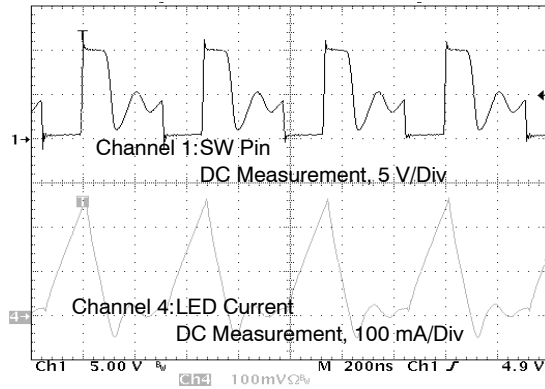
Figure 12. Discontinuous Current Mode (DCM), I OUT = 20 mA
