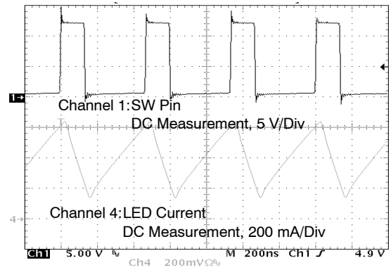
Figure 11. Continue Current Mode (CCM), I OUT = 100 mA
