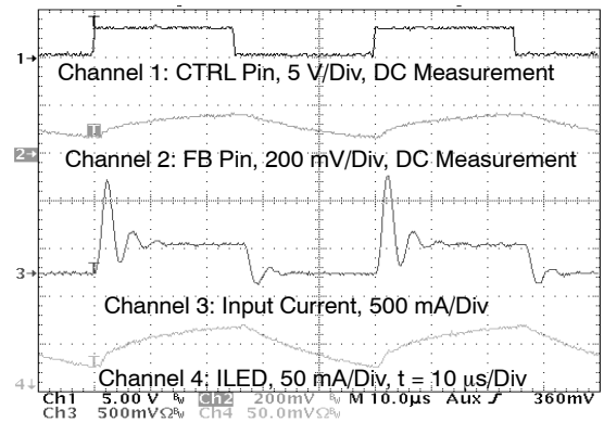
Figure 15. High Frequency Dimming Control, F = 20 kHz
