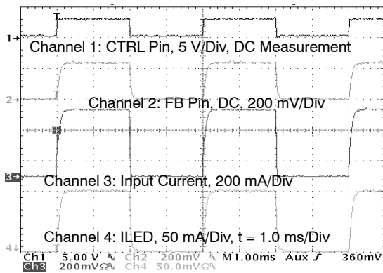
Figure 14. Low Frequency Dimming Control, F = 250 Hz
