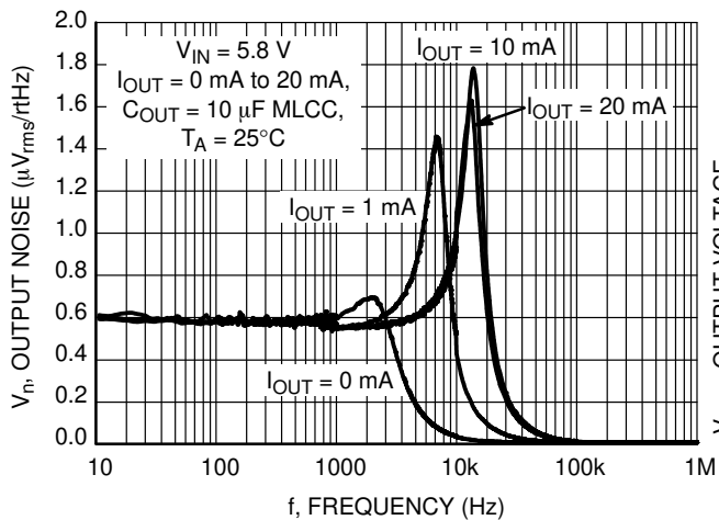
Figure 20. Output Voltage Noise 10 Hz - 1 MHz C OUT = 10 µF
