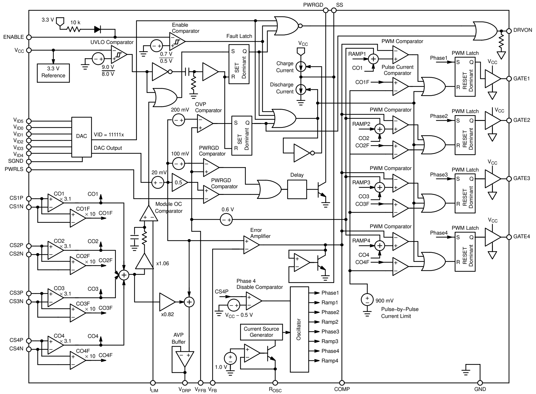
Figure 2. Block Diagram
