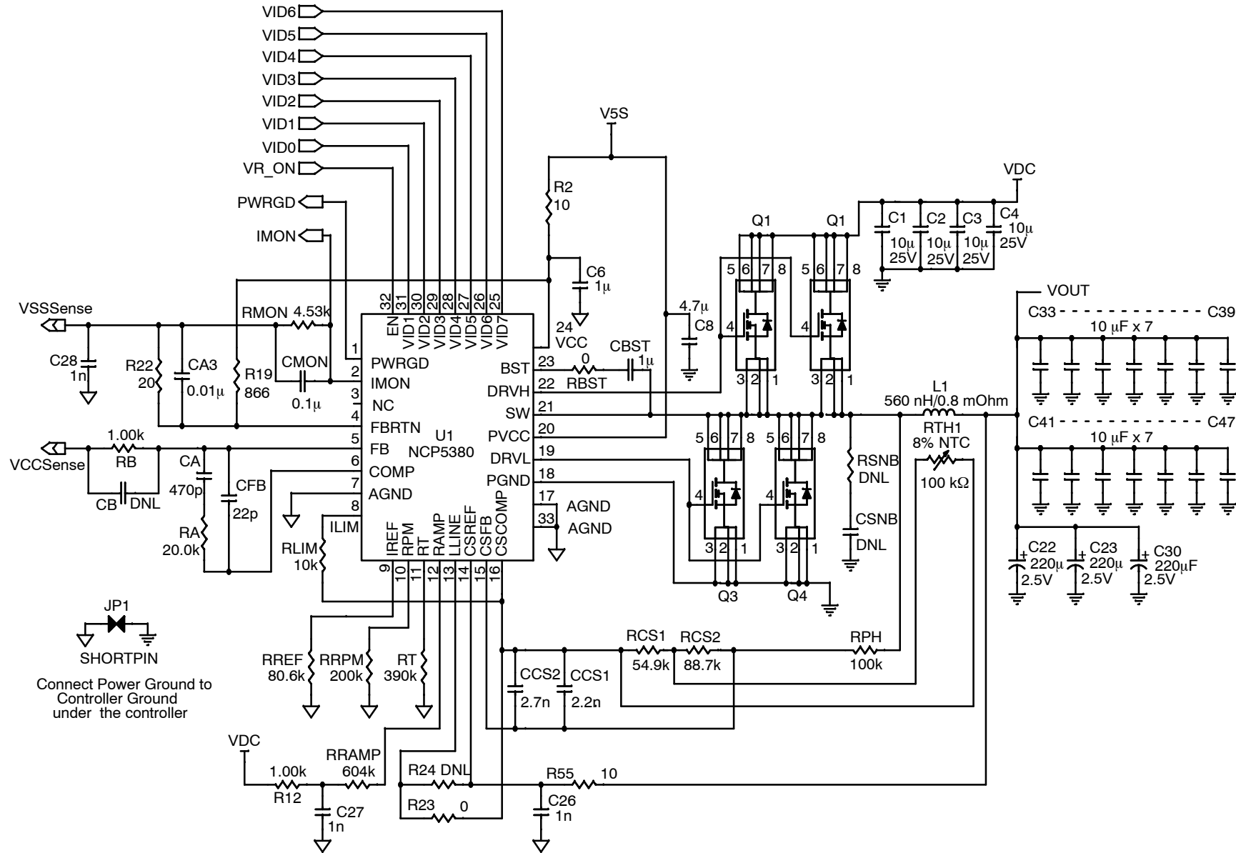
Figure 1. Application Schematic
