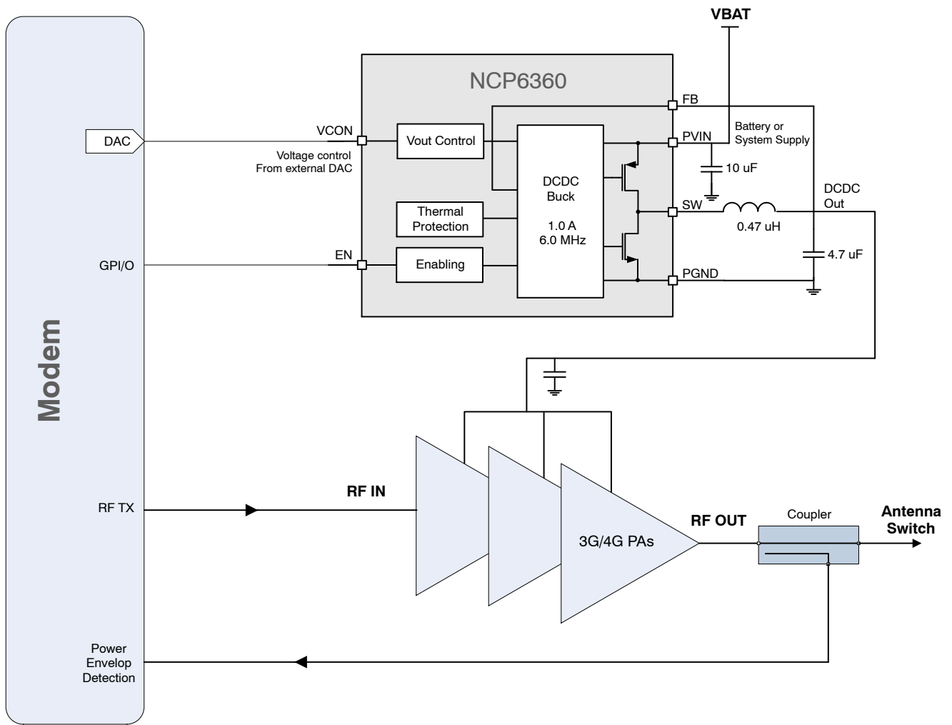
Figure 2. Typical Application
