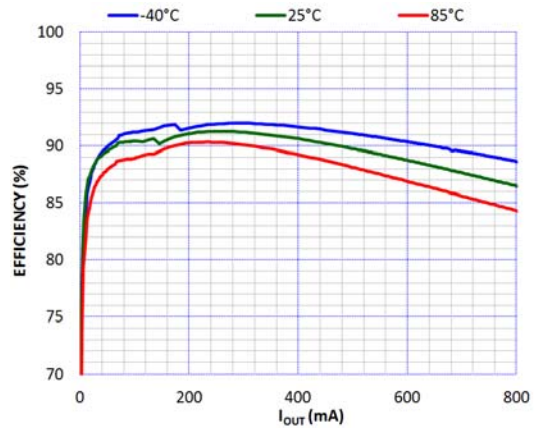
Figure 25. Efficiency vs Output Current vs Temperature PV_{IN} = 4.2\text{ V} , F_{sw} = 3.429\text{ MHz} , V_{OUT} = 1.8\text{ V}
