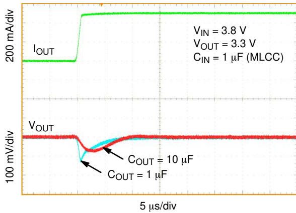
Figure 56. Load Transient Response – Rising Edge, V_{OUT} = 3.3\text{ V} , I_{OUT} = 1\text{ mA} to 500\text{ mA} , C_{OUT} = 1\text{ }\mu\text{F} , 10\text{ }\mu\text{F}
