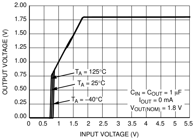
Figure 12. Output Voltage vs. Input Voltage V_{OUT} = 1.8\text{ V}
