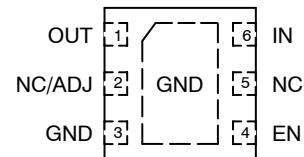
WDFN6 2x2 mm (Top View)
