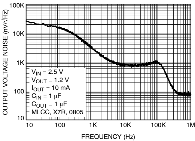
Figure 13. Output Voltage Noise Spectral Density for V_{OUT} = 1.2 V , I_{OUT} = 10 mA , C_{OUT} = 1 \mu F
