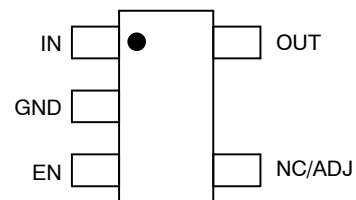
TSOT-23-5 (Top View)
