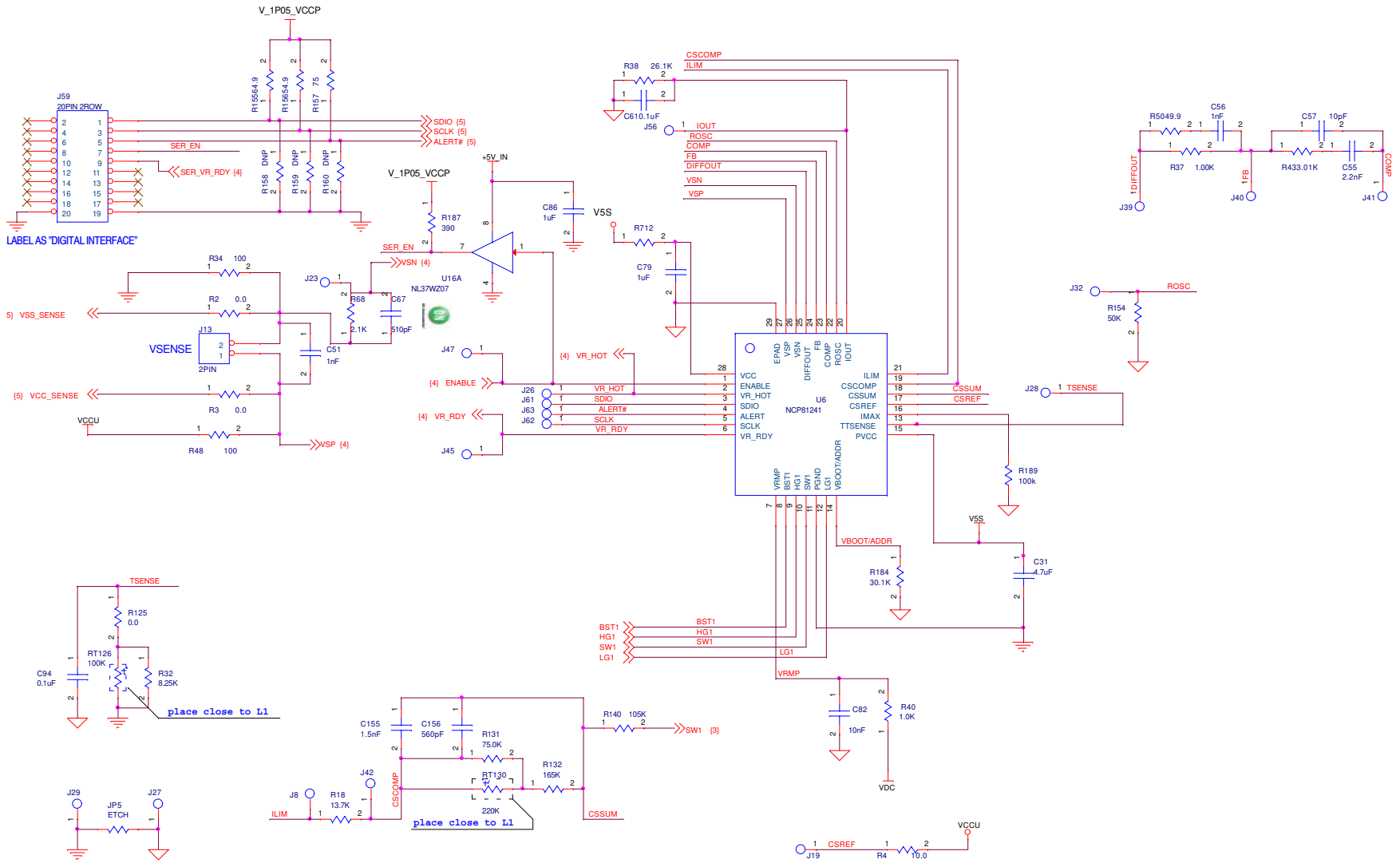
Figure 2. Controller Application Schematic
