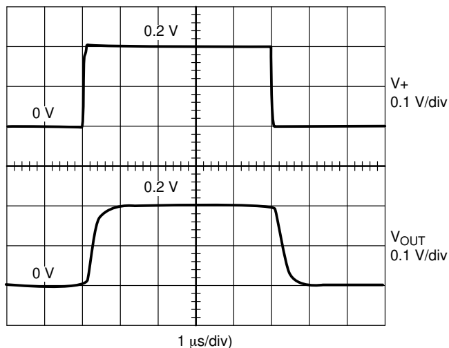
Figure 7. Slew Rate
