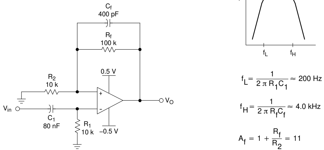
Figure 37. 1.0 V Voiceband Filter
