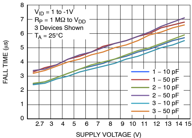
Figure 14. Output Fall Time vs. Power Supply
