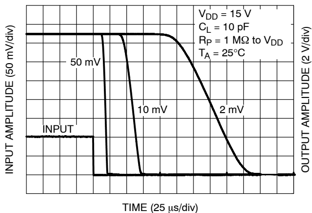
Figure 13. Propagation Delay H-L (15 V)
