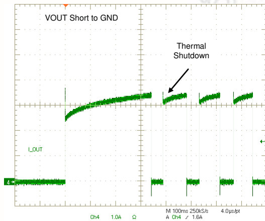
Current Limit Test (VIN=2.5V)
