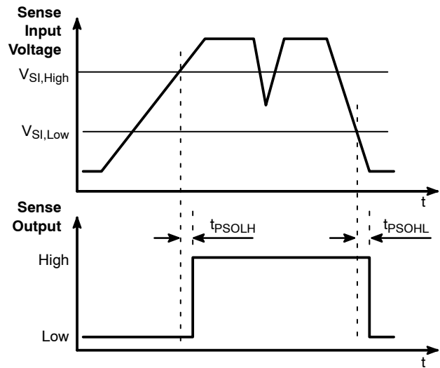
Figure 36. Sense Timing Diagram
