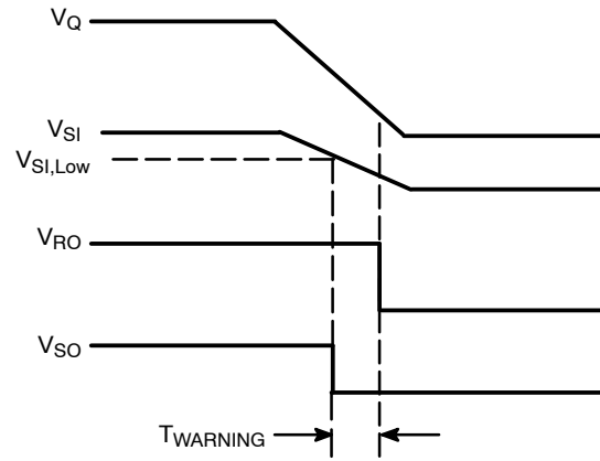
Figure 35. SO Warning Timing Waveform
