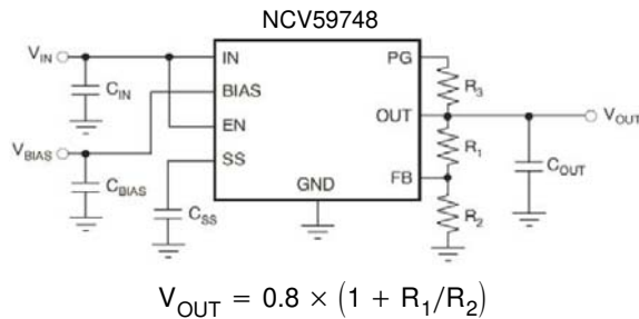
Figure 16. Typical Application Schematics
