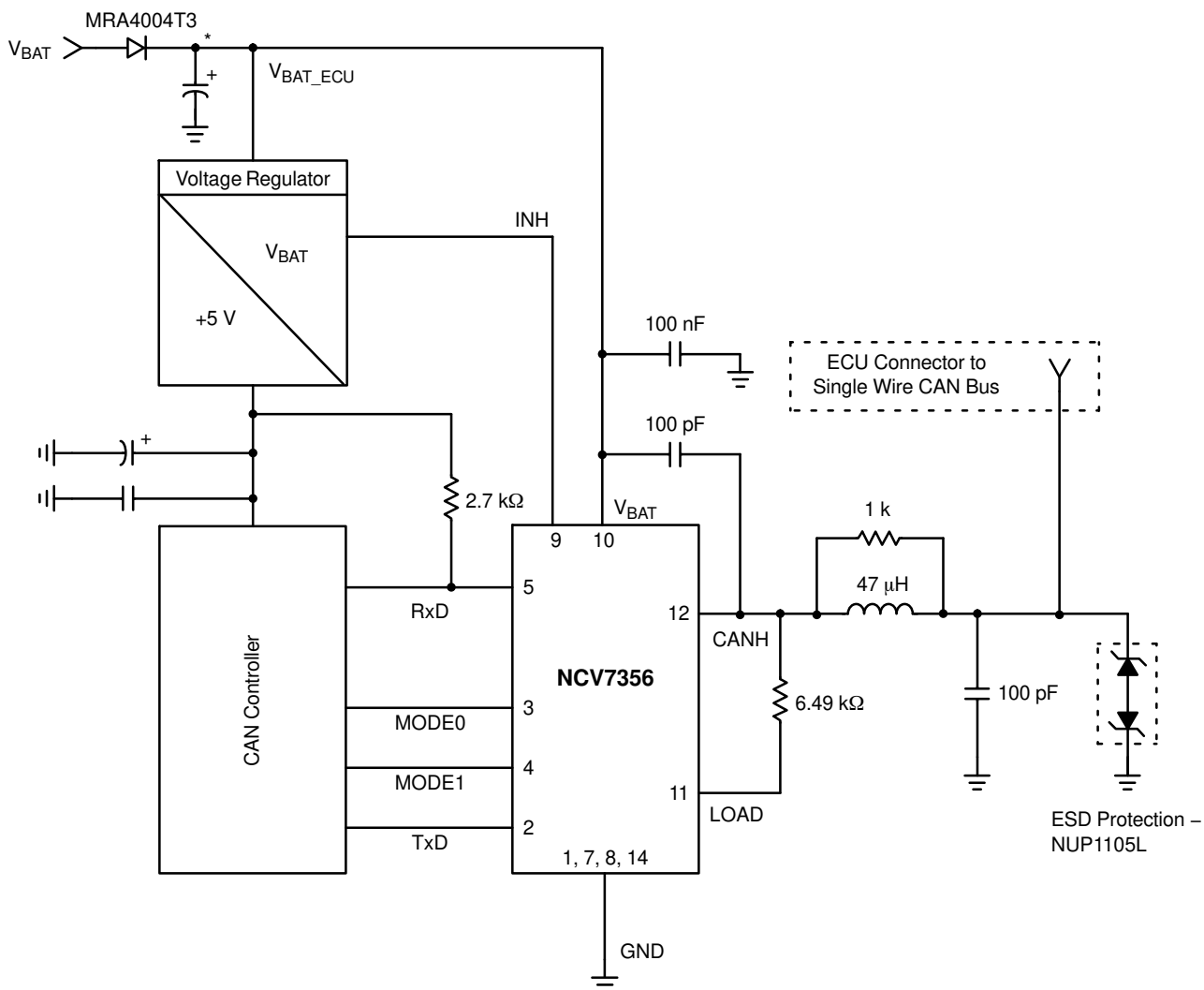
Figure 12. Application Circuitry, 14 Pin Package
