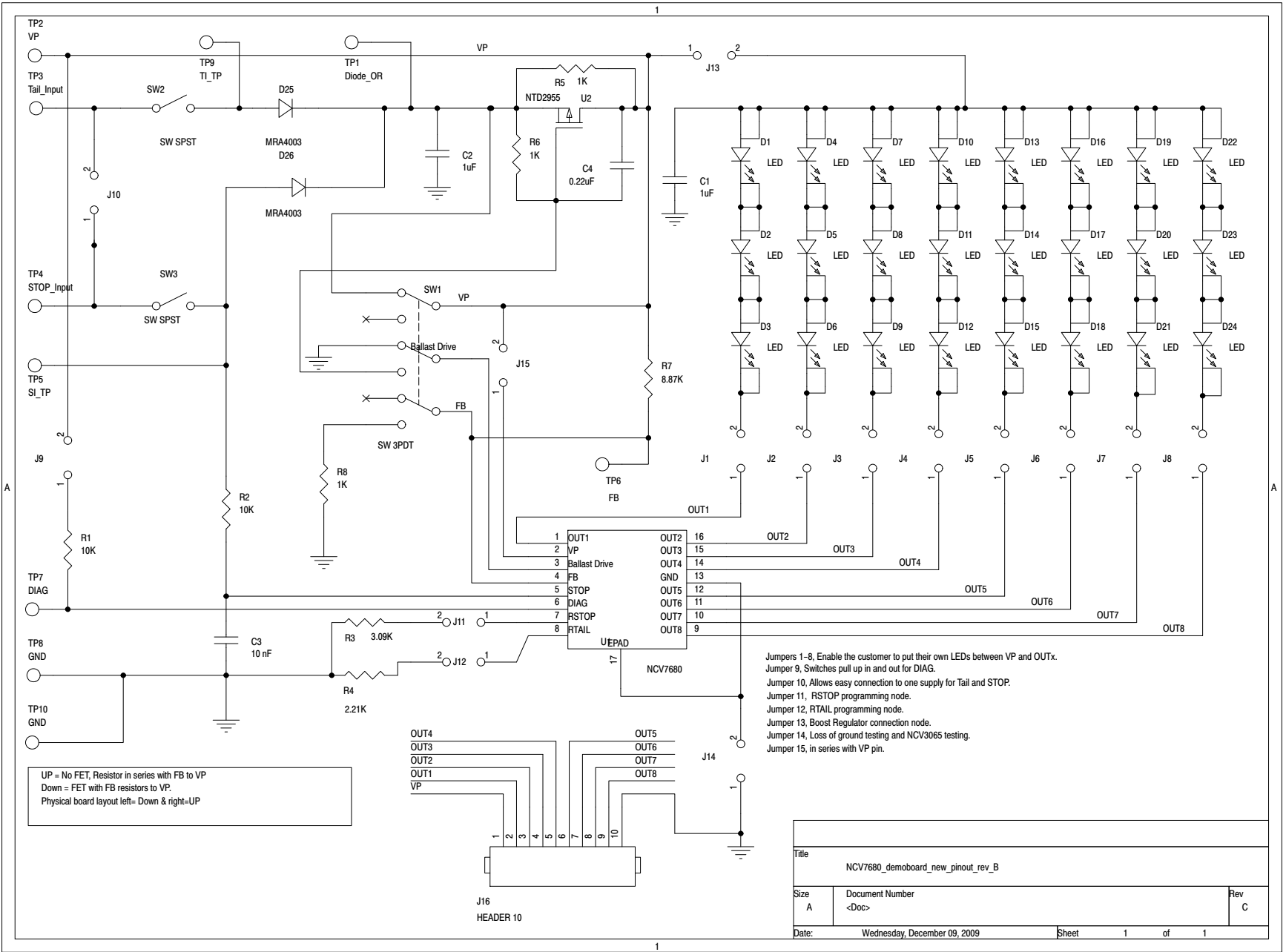
Figure 2. NCV7680PWR22GEVB Schematic
