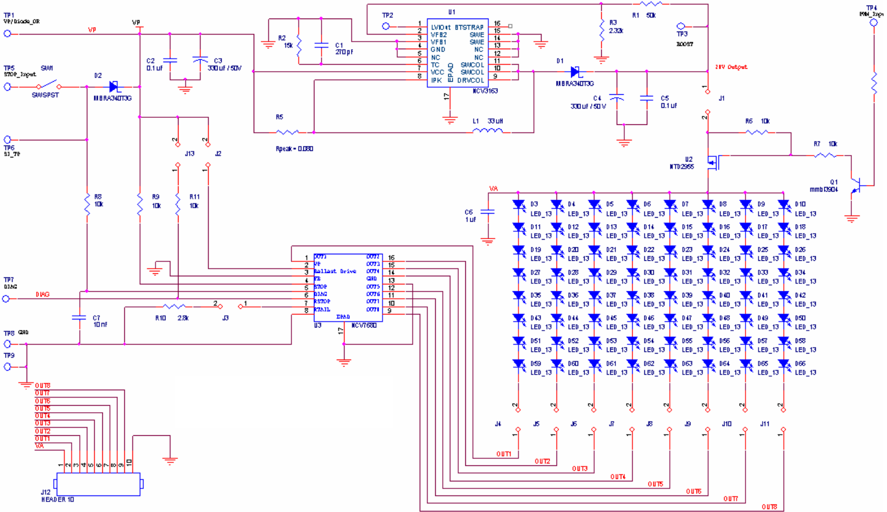
Figure 2. NCV7680-NCV3136EVB Schematic
