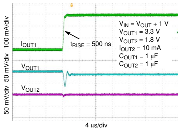
Figure 44. Load Transient Response – 3.3 V – Rising Edge, I_{OUT1} = 1 \text{ mA} to 300 mA
