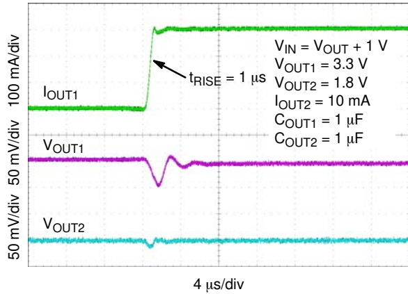
Figure 36. Load Transient Response – 1.8 V – Rising Edge, I_{OUT1} = 100 \mu\text{A} to 300 mA
