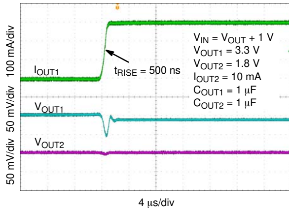
Figure 38. Load Transient Response – 1.8 V – Rising Edge, I_{OUT1} = 1 \text{ mA} to 300 mA
