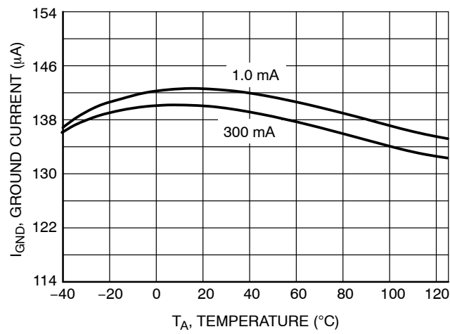
Figure 8. Ground Current vs. Temperature
