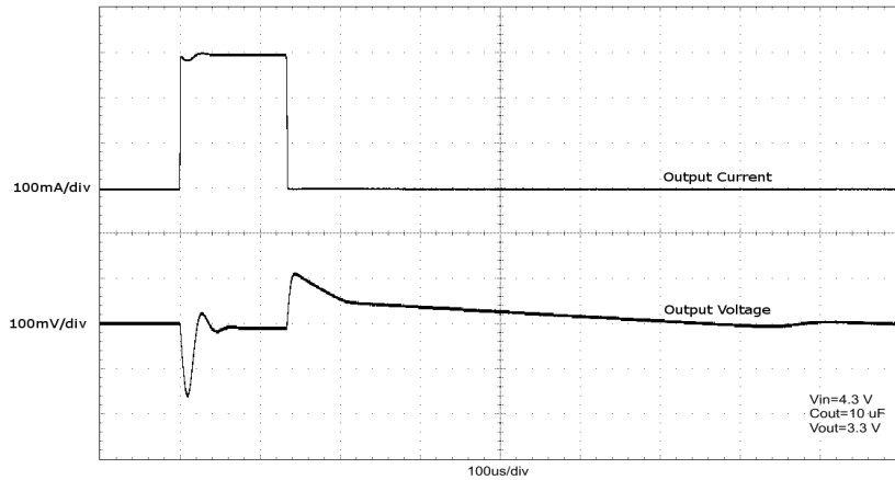
Figure 18. Load Transient Response ( 10\ \mu\text{F} )
