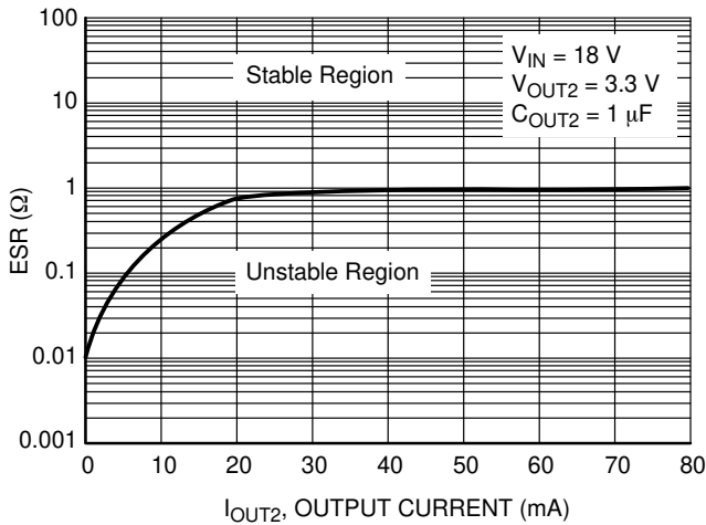
Figure 24. C OUT2 ESR Stability Region – 1 μF
