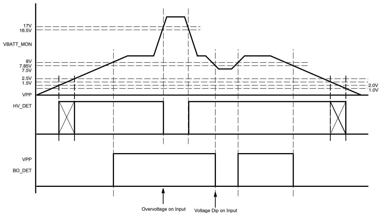
Figure 8. Warning Circuitry Timing Diagram
