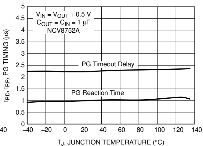
Figure 76. NCV8752A PG Reaction Time, Delay Timing
