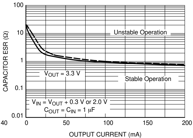
Figure 78. Stability vs. Output Capacitors ESR
