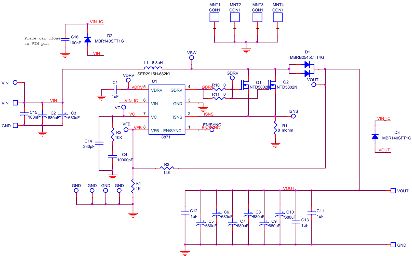
Figure 7. NCV8871BSTGEVB Evaluation Board Schematic
