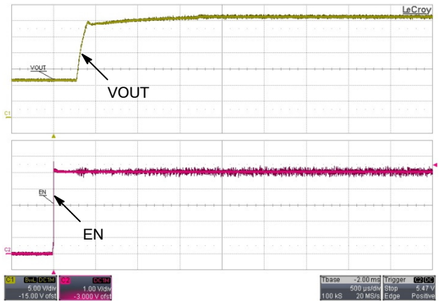
Figure 4. Typical Start-up with V_{IN} = 12\text{ V} , 10 LEDs/60 mA
