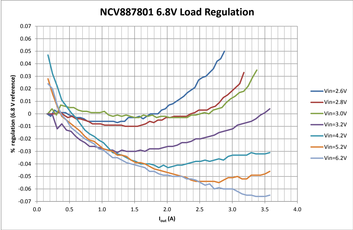
Figure 9 NCV887801 Load Regulation
