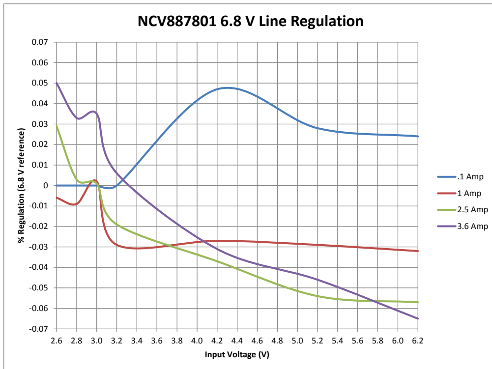
Figure 8 NCV887801 Line Regulation
