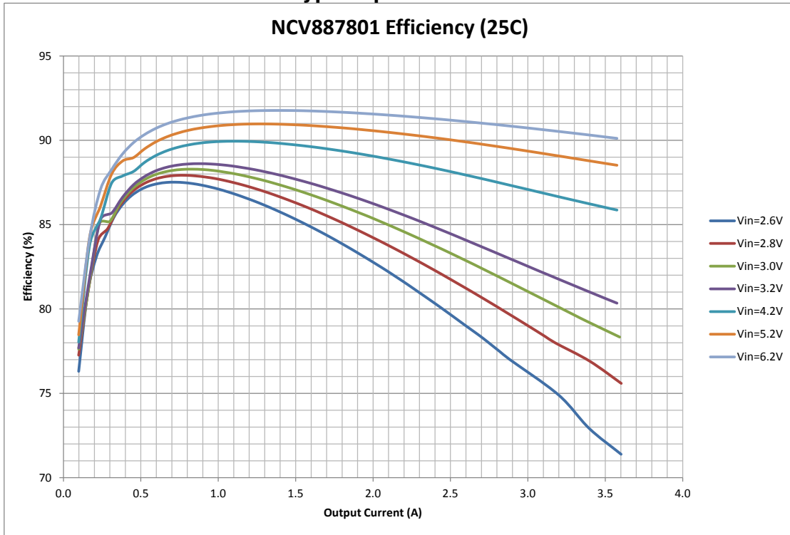
Figure 7 NCV887801 Efficiency
