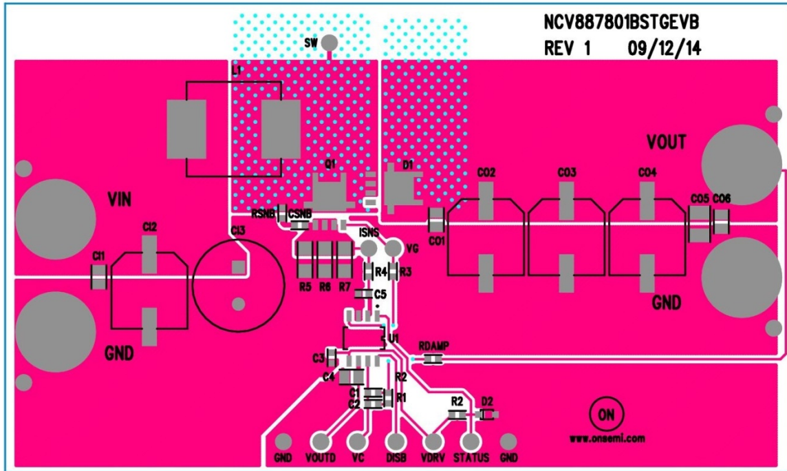
Figure 5. Top View
