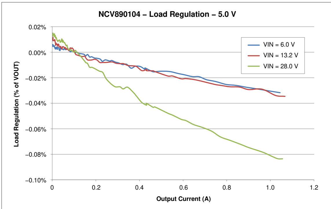
Figure 13. Load Regulation with a 5.0 V Output
