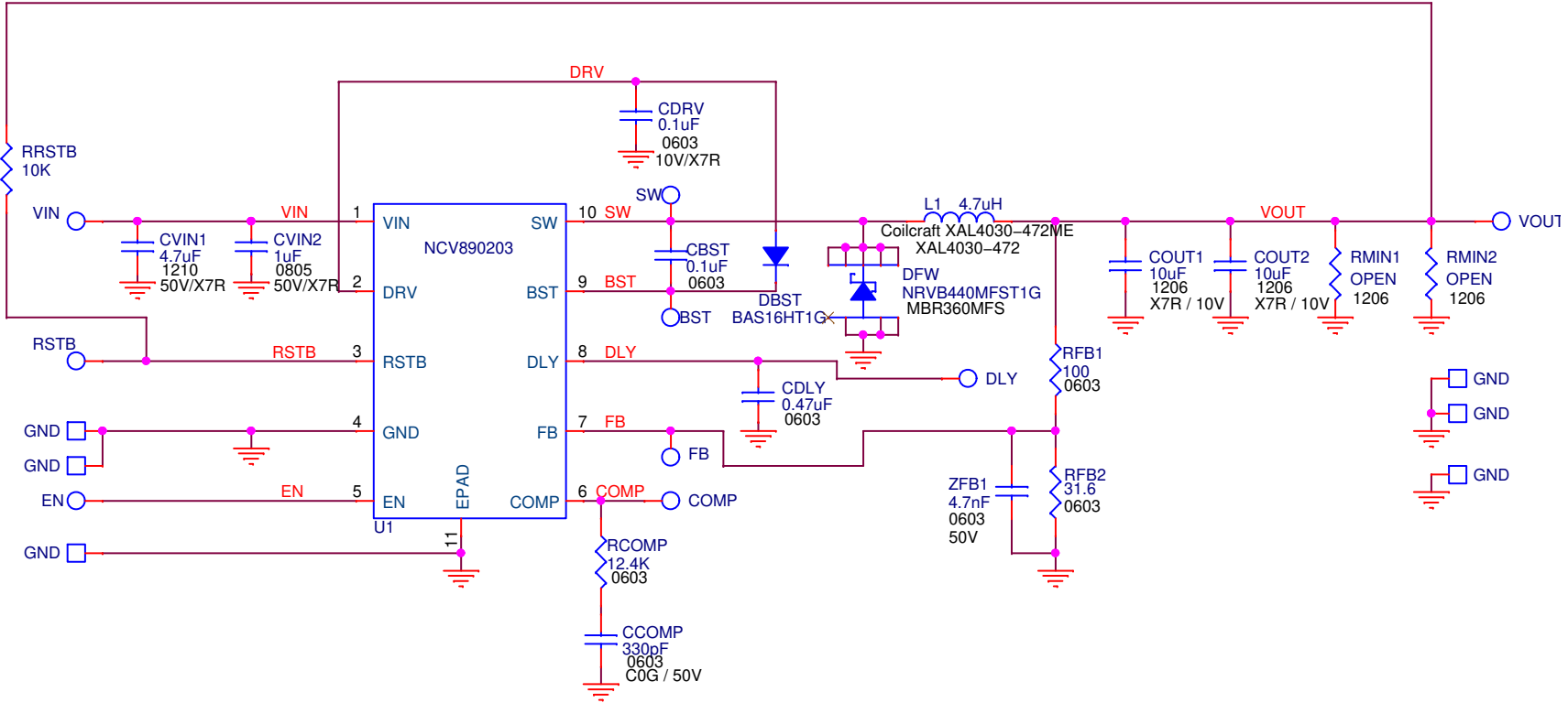
Figure 13. Schematic
