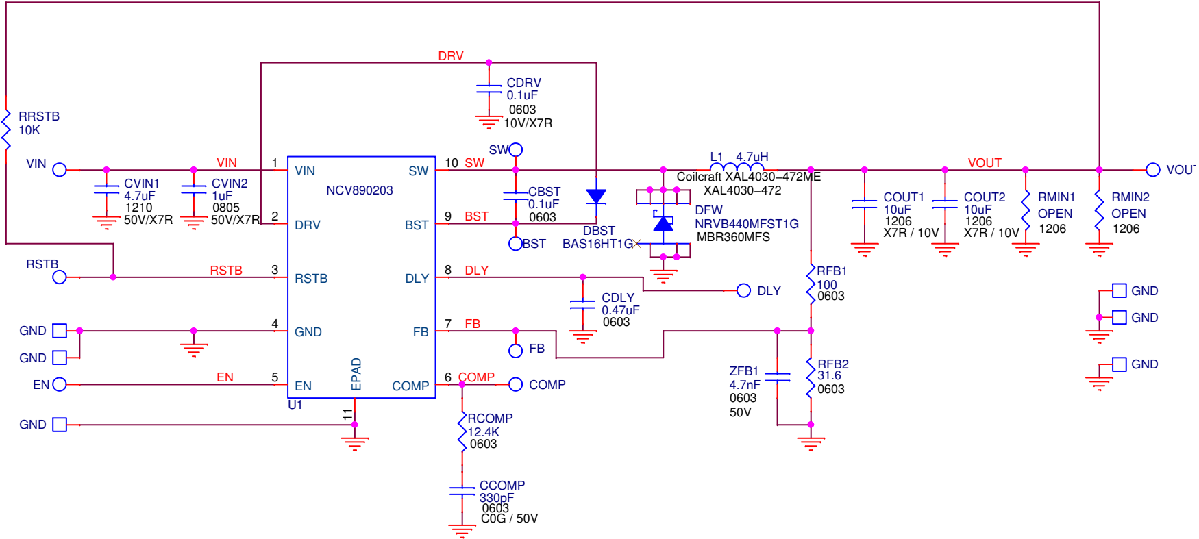
Figure 4. NCV890203GEVB Evaluation Board Schematic
