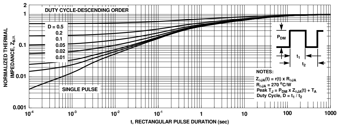
Figure 17. Transient Thermal Response Curve. Note : Thermal characterization performed using the conditions described in note 1b. response will change depending on the circuit board design.
