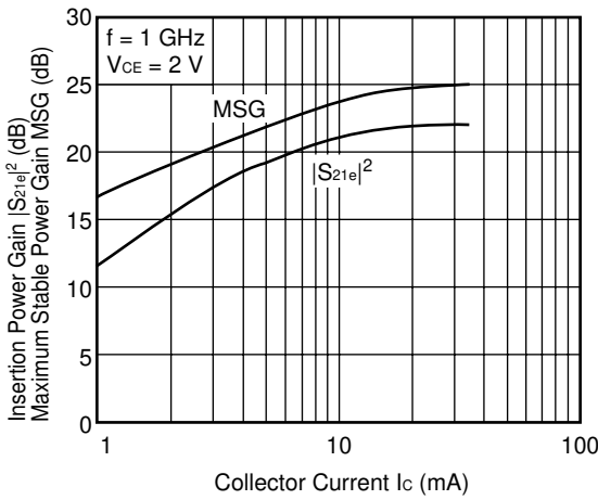
INSERTION POWER GAIN, MSG vs. COLLECTOR CURRENT
