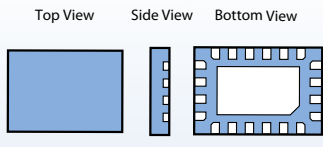
T5R Package (3.5 x 2.5 x 0.55)
