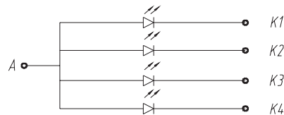
LED Source(CIRCUIT DIAGRAM)
