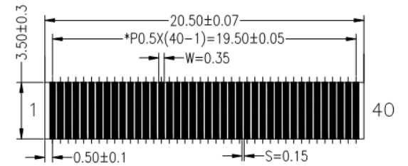
DETAIL B
