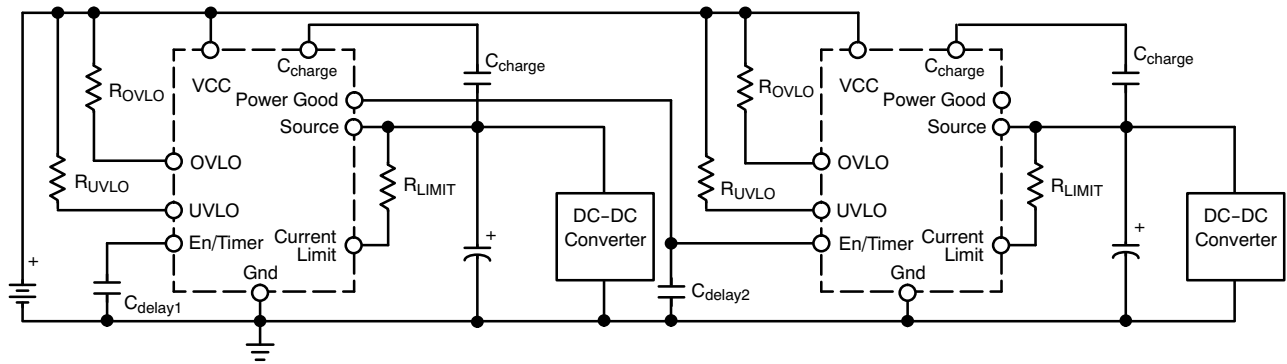
Figure 16. Turn-on Sequencing Using Power Good Signal
