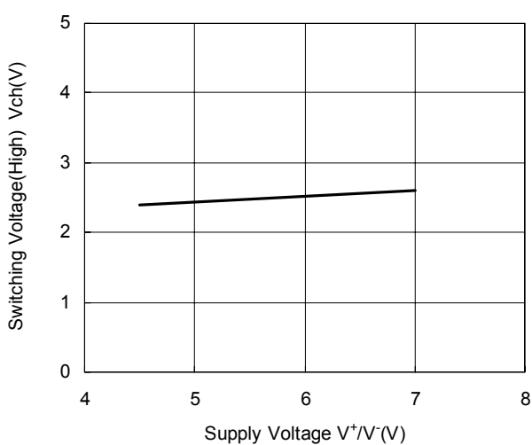
Switching Voltage(High) vs. Supply Voltage ( T_a=25^\circ\text{C} )
