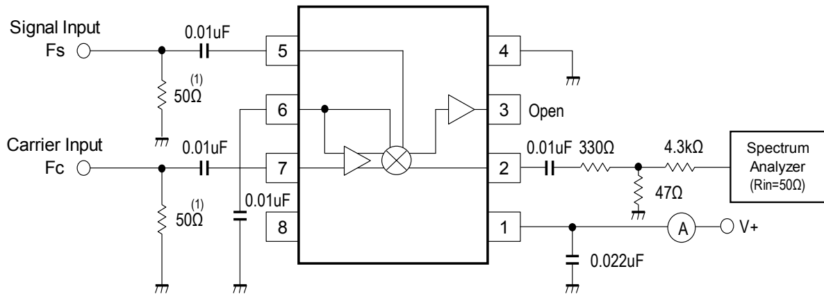
TEST CIRCUIT 2
