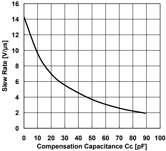
Slew Rate vs. Compensation Capacitance T_a=25^\circ C
