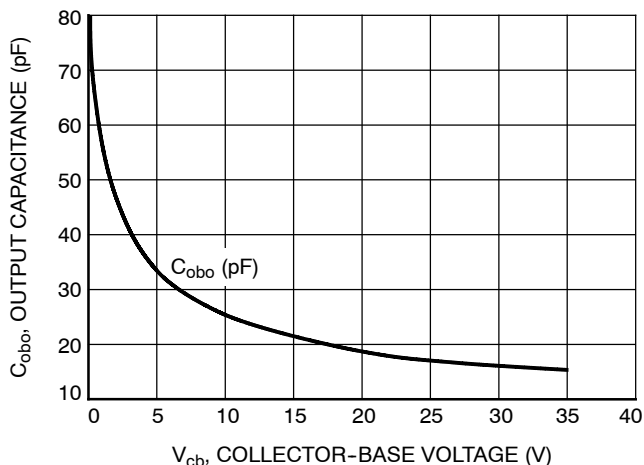
Figure 8. Output Capacitance
