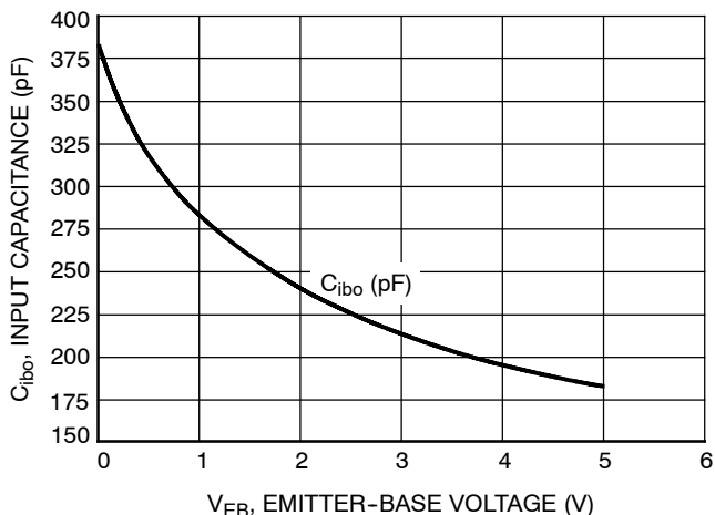
Figure 7. Input Capacitance
