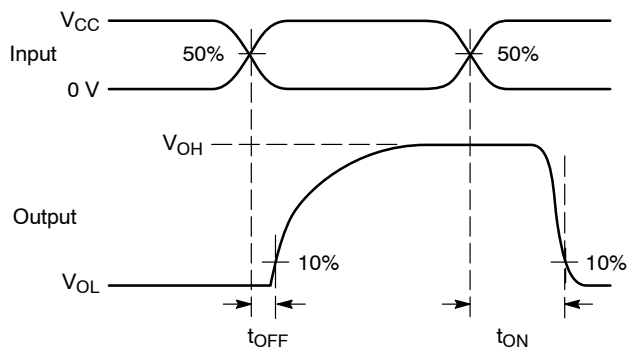
Figure 5. t_{ON}/t_{OFF}
