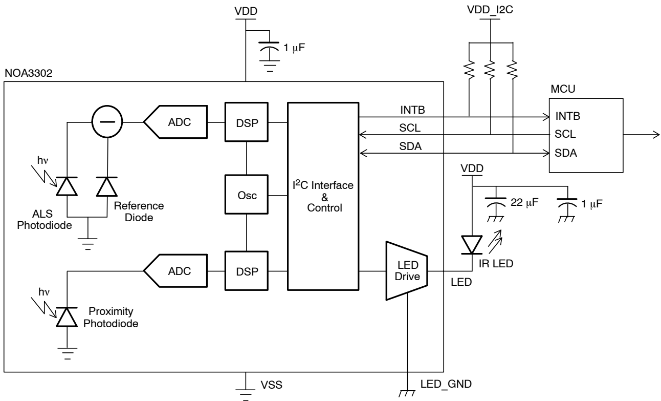
Figure 1. NOA3302 Application Block Diagram
