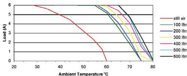
THERMAL DERATING
