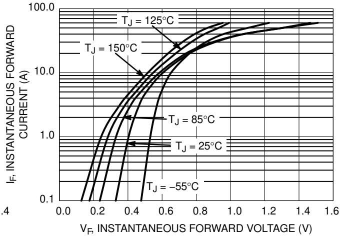
Figure 2. Maximum Instantaneous Forward Characteristics
