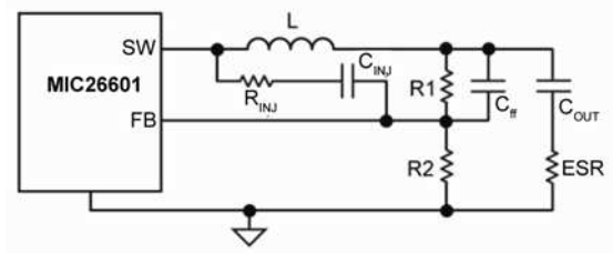
Figure 5c. Invisible Ripple at FB
