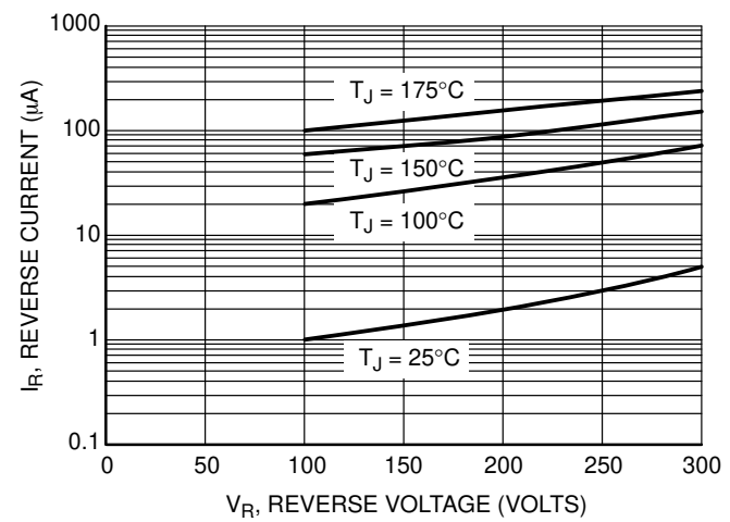
Figure 4. Maximum Reverse Current for MURS230T3G, NRVUS230T3G
