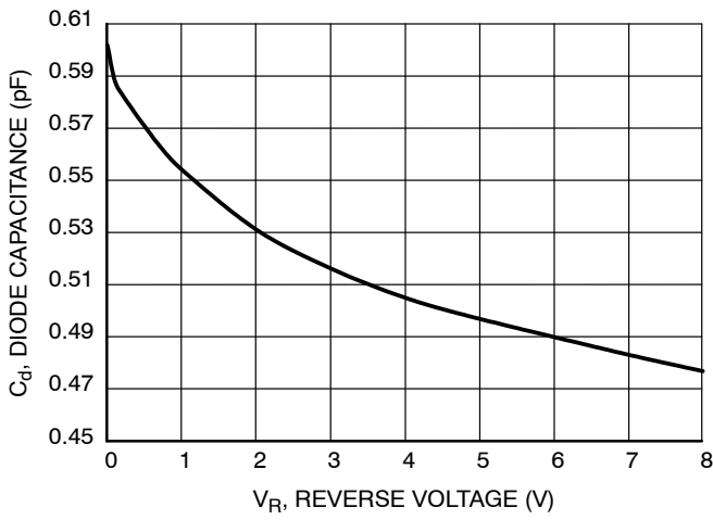
Figure 14. Capacitance
