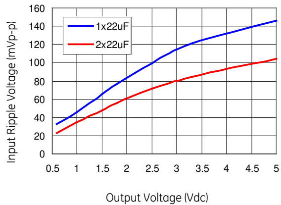
Figure 46. Input ripple voltage for various output voltages with 1 \times 22 \mu F or 2 \times 22 \mu F ceramic capacitors at the input (6A load). Input voltage is 12V.
