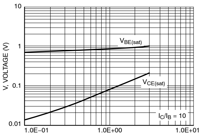
Figure 4. "ON" Voltages
