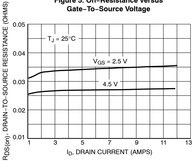
Figure 7. On-Resistance versus Drain Current and Gate Voltage
