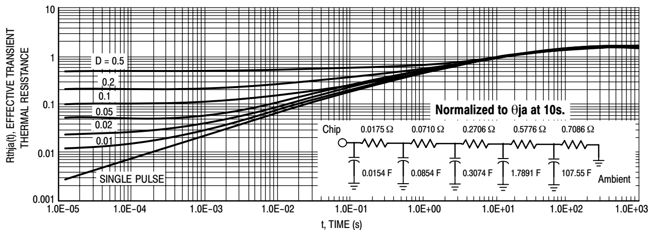
Figure 24. Thermal Response
